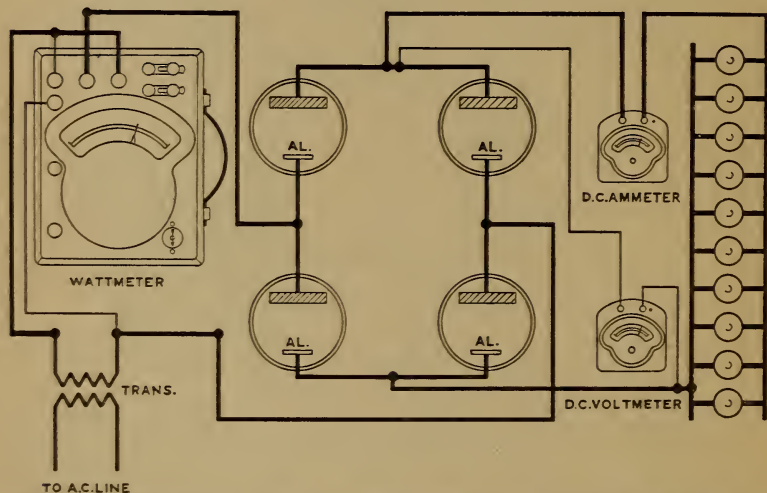
FIG. 24.—EFFICIENCY TEST OF AN ELECTROLYTIC CURRENT RECTIFIER.
